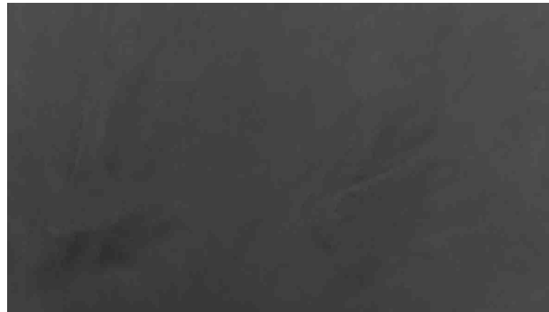
Slate
